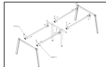
CROSS BEAM & LEG ASSEMBLY REMOVAL
